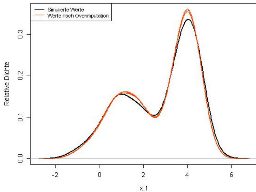
Abbildung 1: Comparison of the overimputations via density plots, Amelia 1.6.1 (at the top) and Amelia 1.7 (at the bottom)
